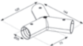
COSMOS-Y-19
