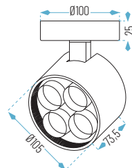
HERA-FS2-19-24W
