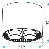
HERA-R1-19-24W
